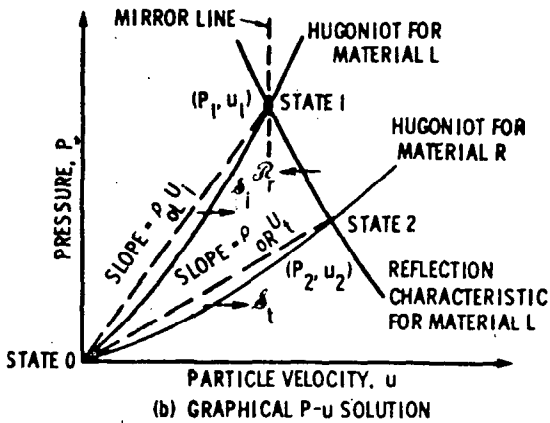
(b) GRAPHICAL P-u SOLUTION
